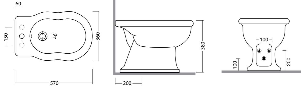
BOHEME BIDET cod. 28220101 Bidet boheme, rubinetteria mono/tre fori. Bidet boheme single/three tap holes.
