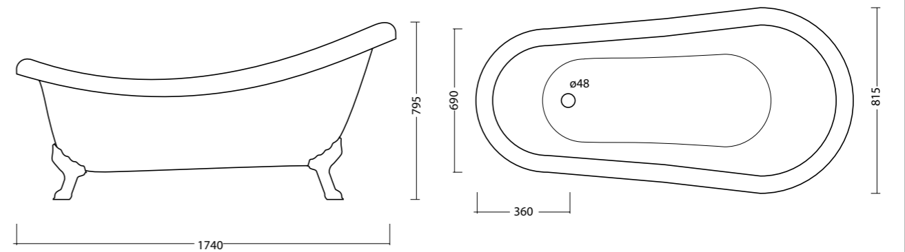
BOHEME VASCA cod. VAB0 Vasca boheme in acrilico 175x81. Acrylic boheme bathtube 175x81.
